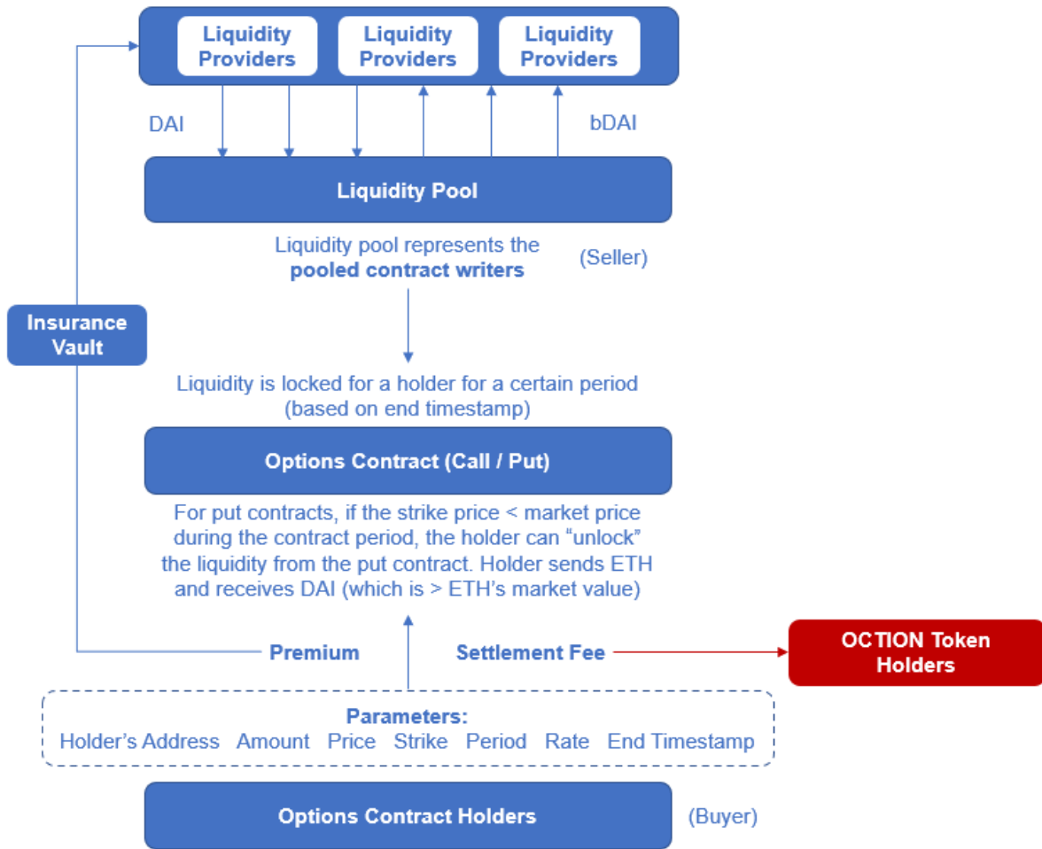
Figure 3: The OCTION Ecosystem
